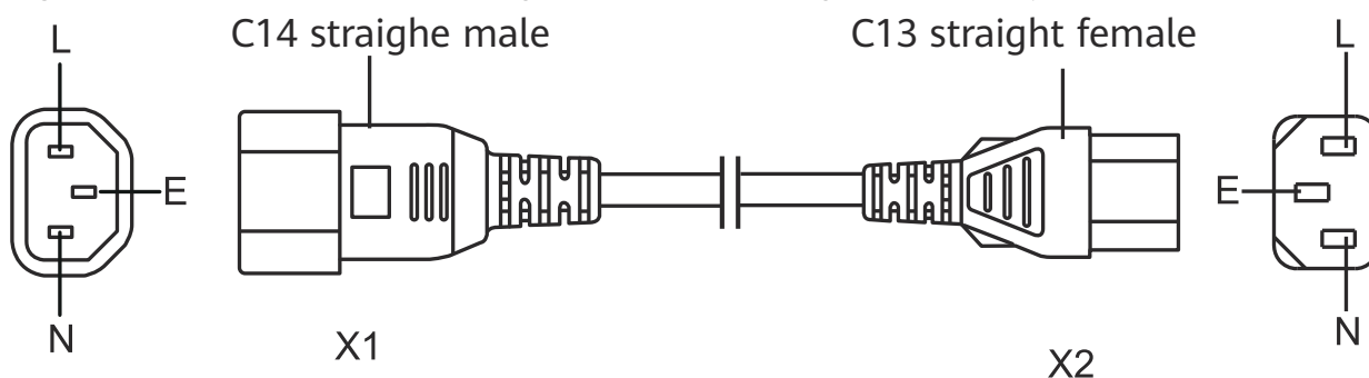
Figure 6-14 Structure of a C14 straight male to C13 straight female AC power cable
