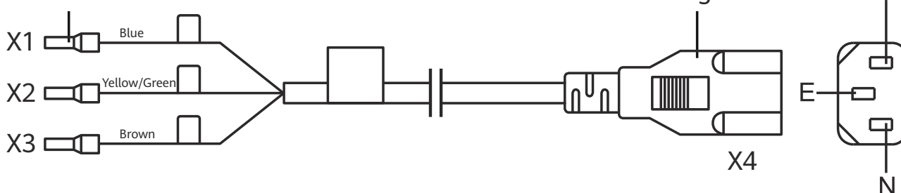
Figure 6-16 Structure of a Cord end to C13 straight female AC power cable (used in China)
