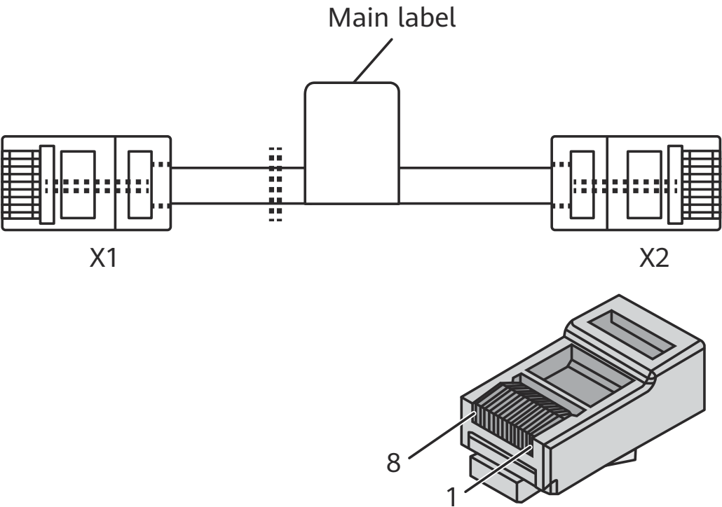
Figure 6-4 Structure of an Ethernet cable
